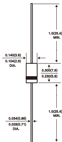
Dimensions in inches and (millimeters)
