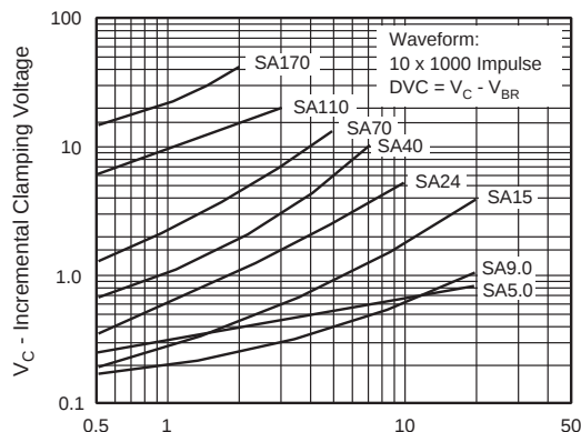
Fig. 8 - Incremental Clamping Voltage Curve Uni-Directional
